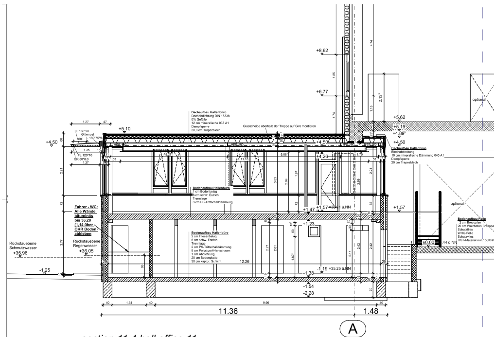
section 11.4 hall office 11
