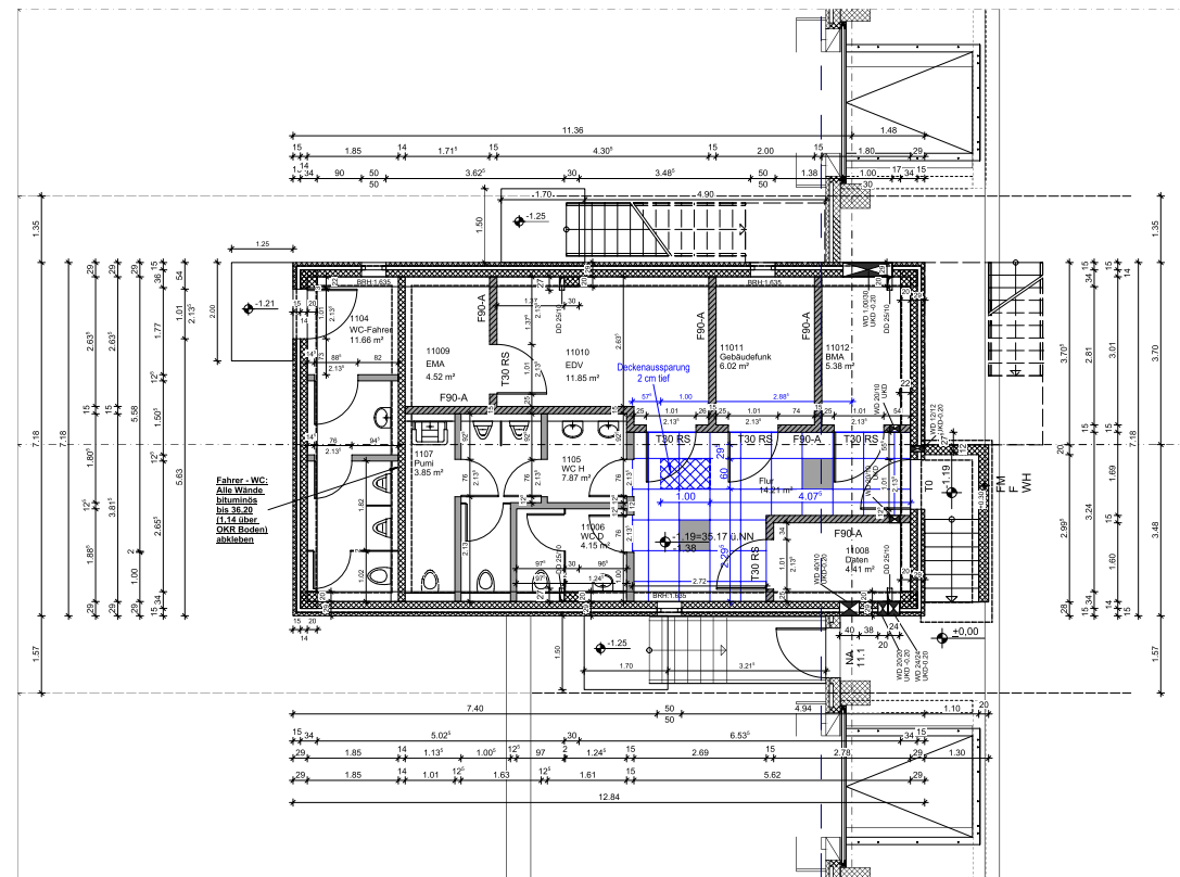
layout ground floor hall office (B11)
