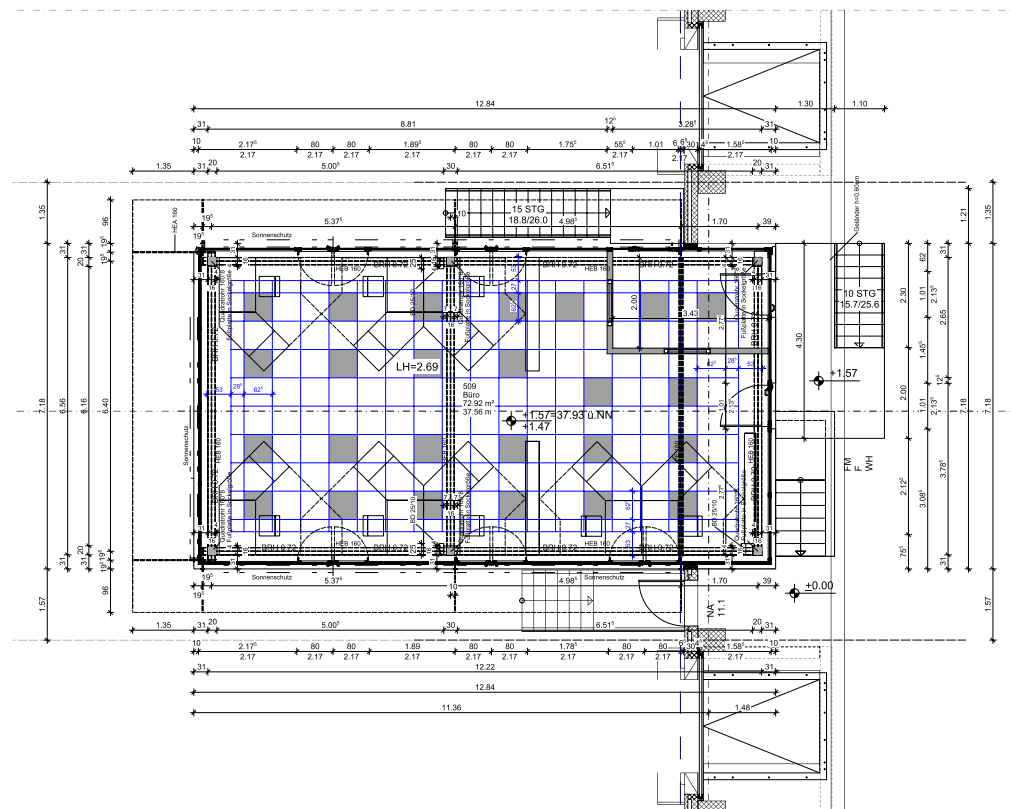
layout 1st floor hall office (B11)
