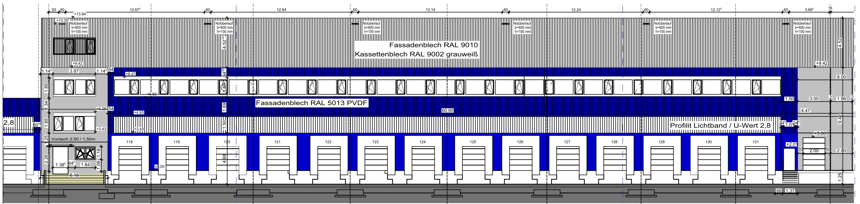
detail of implementation plan elevations hall 10
