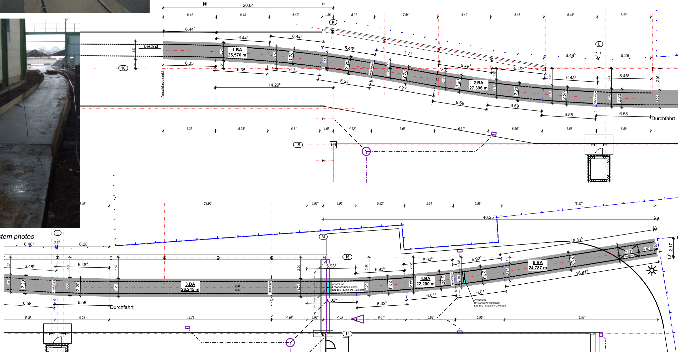
details of the implementaion plan for the track foundation slab
