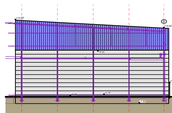
view section 16'
