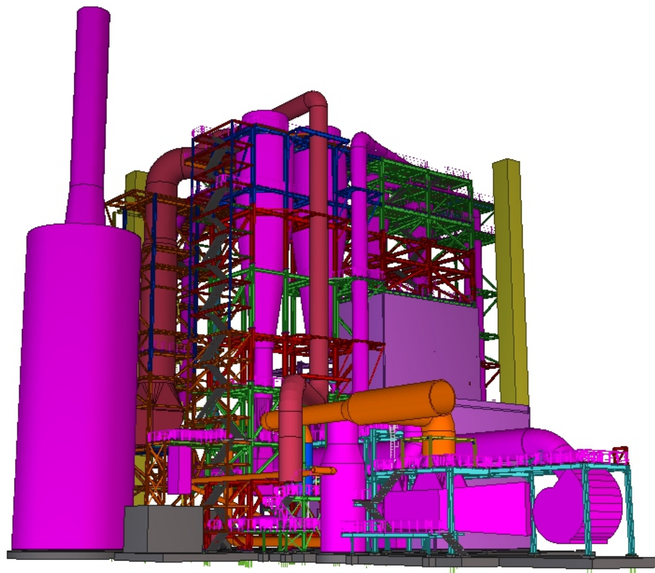
rendered model of the dryer framework
