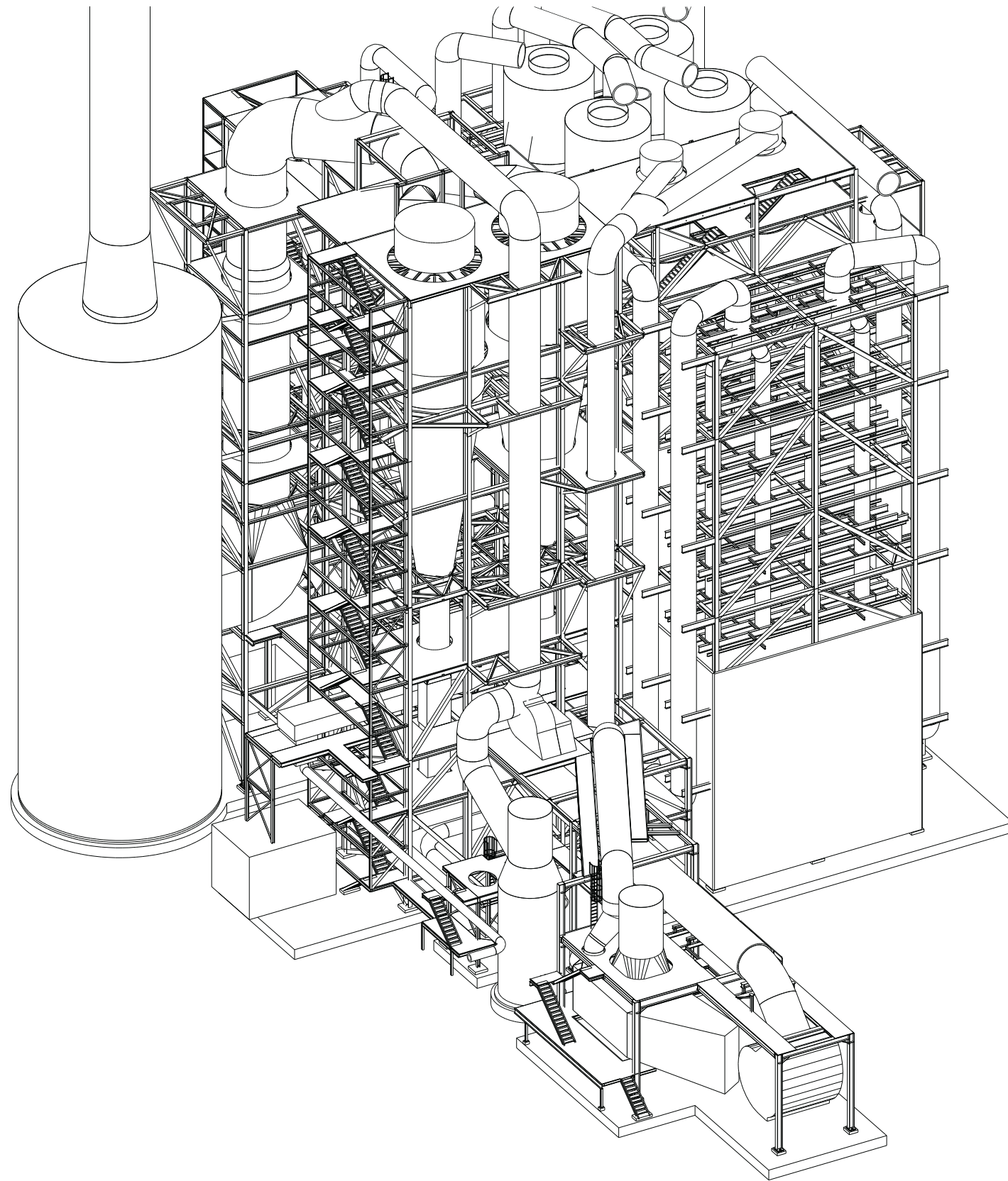
isometry 1
