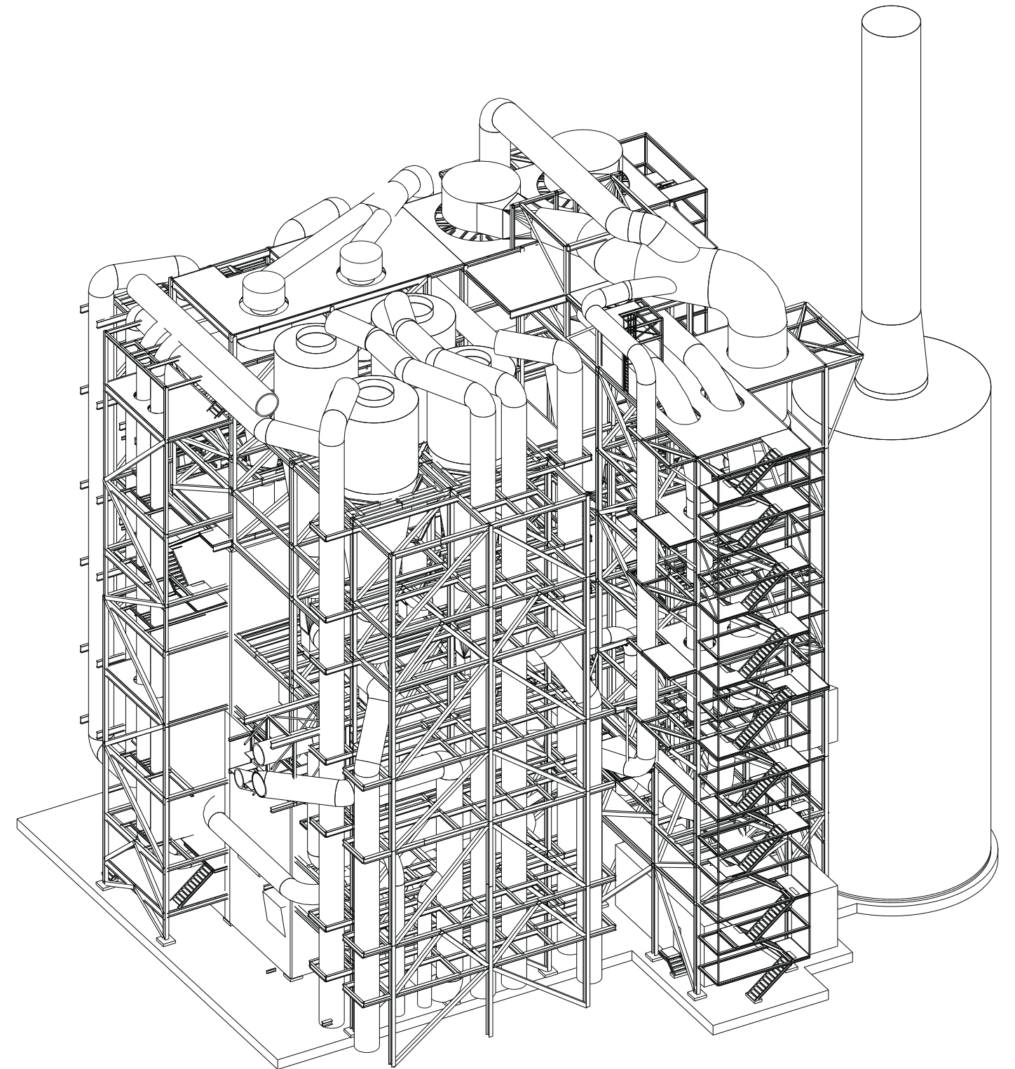
isometry 2
